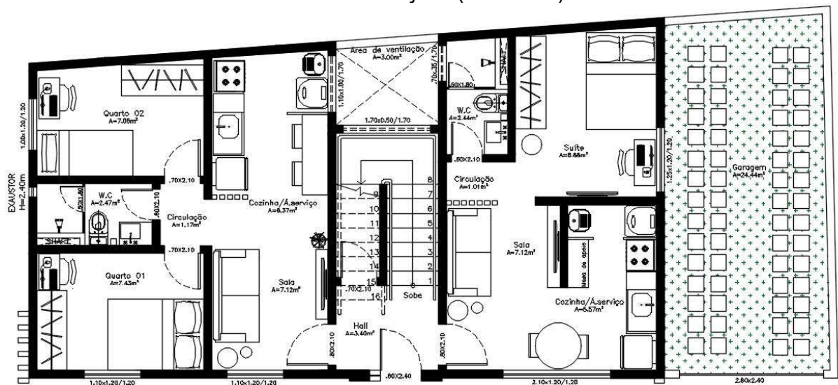
Kitnet – Layout (AutoCAD)
